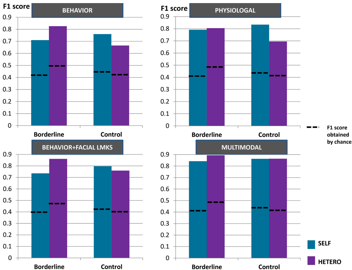
Fig. 3. Prediction of stress (F1 score) using machine learning based on unimodal and multimodal features according to perception (hetero- vs. self-perception) and clinical status (BPD vs. HC).
